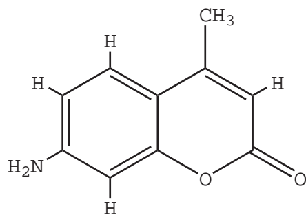
7-Amino-4-methylcoumarin
