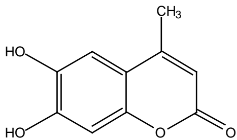
4-Methylesculetin
