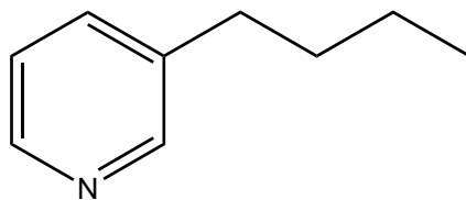
3-n-Butylpyridine
