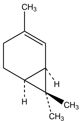
2-Carene
