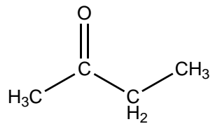
2-Butanone
