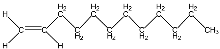
1-Dodecene
