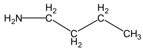
n-Butylamine
