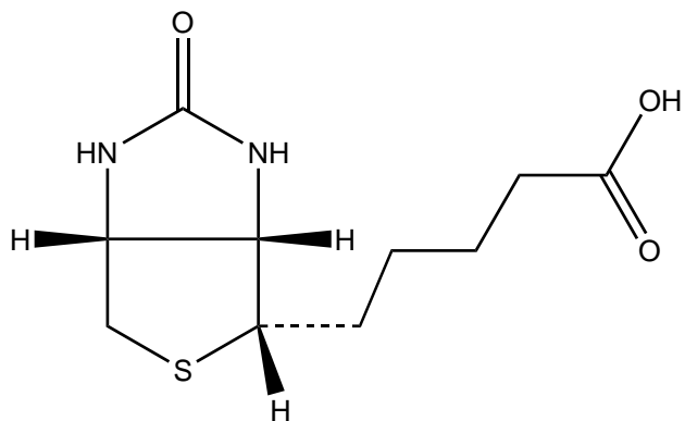
(+)-Biotin
