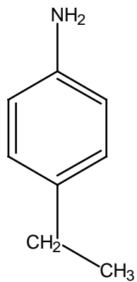
4-Ethylaniline
