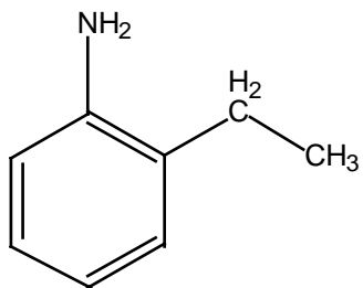
2-Ethylaniline
