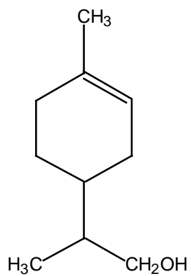
Menth-1-en-9-ol
