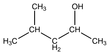
4-Methyl-2-pentanol
