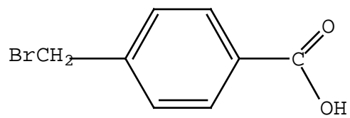
p-Bromomethylbenzoic acid
