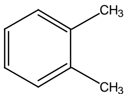
o-Xylene
