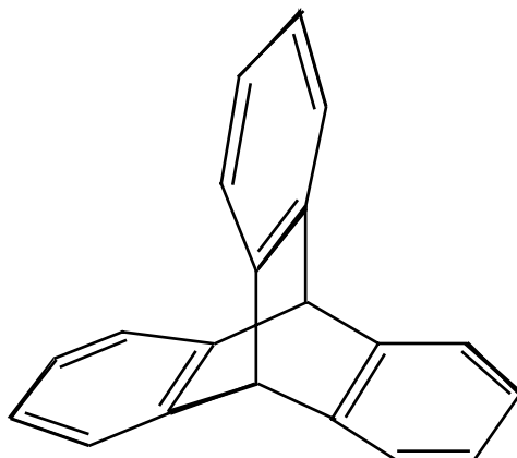
Triptycene
