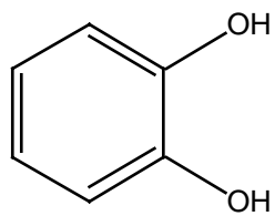
Pyrocatechol
