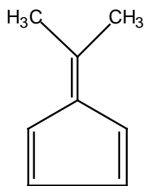
Dimethylfulvene
